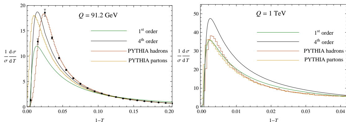
Figure 12: Comparison between theoretical predictions in effective field theory at first order and fourth order, as defined in table 1, and PYTHIA at the parton and hadron level. ALEPH data is included in the first panel.
