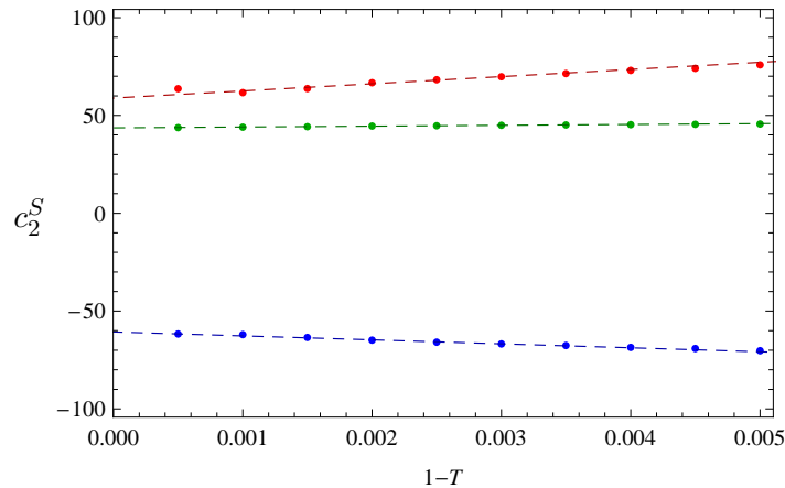
Figure 3: Extraction of the two-loop constants in the soft function. The points correspond to the value of an infrared cutoff applied to the fixed-order calculation. The lines are interpolations among the points from \tau = 0.001 to \tau = 0.003 extrapolated to \tau = 0 to extract the constants. From top to bottom, the curves are the C_F^2 , C_A and n_f color factors.
